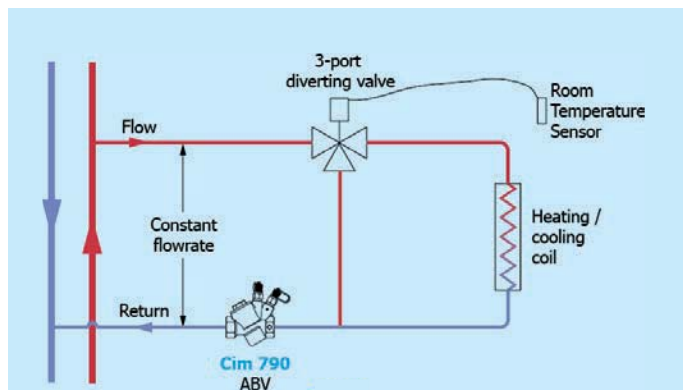
Figure 34 CFR in constant volume systems
