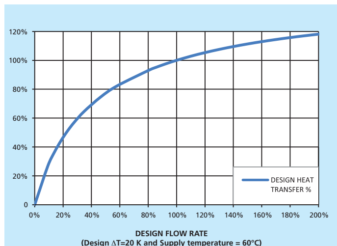
Figure 3 Effects of extra flows
