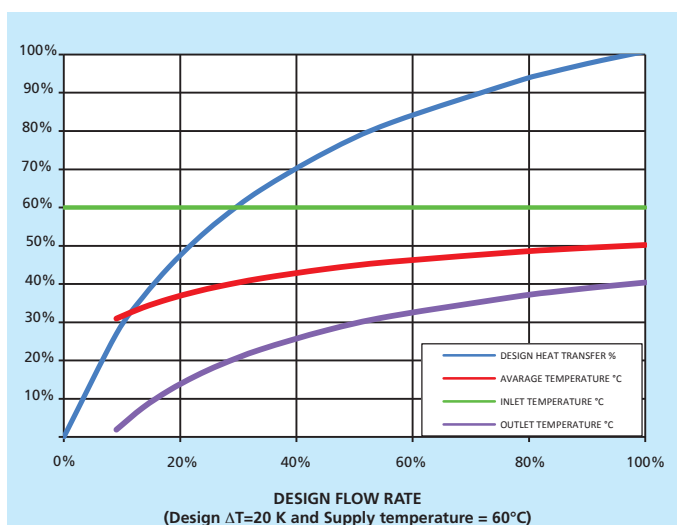
Figure 1 Effects of flow variation
