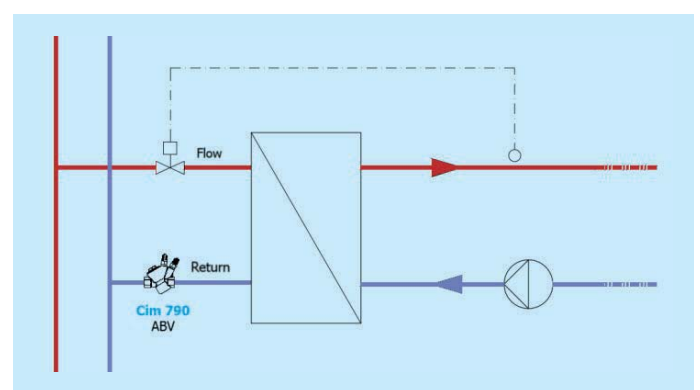
Figure 38 CFR with heat exchanger
