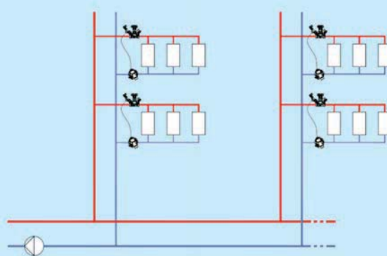
Figure 44 Differential pressure valve on the manifold
