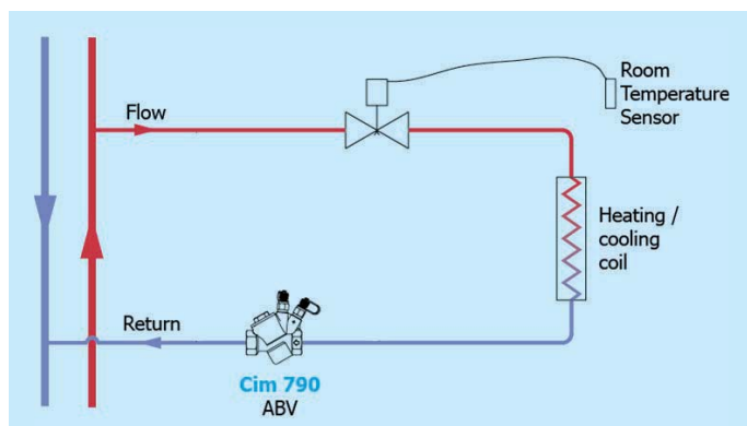
Figure 35 CFR in variable volume systems
