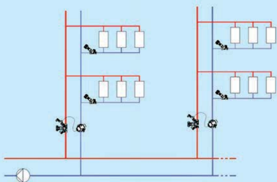
Figure 43 Differential pressure valve on the riser
