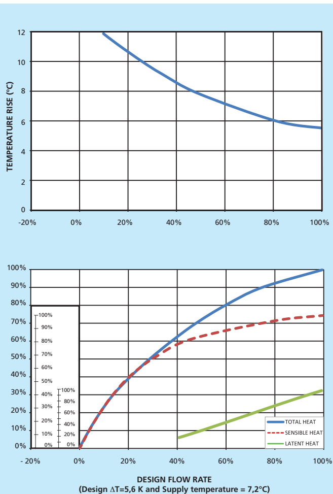
Figure 4 Effects of flow variation in cooling systems
